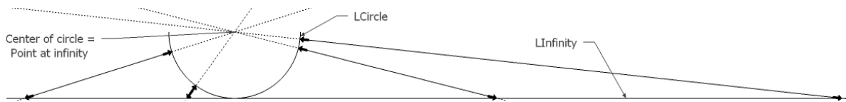
FIGURE 3. Stereographic projection.
