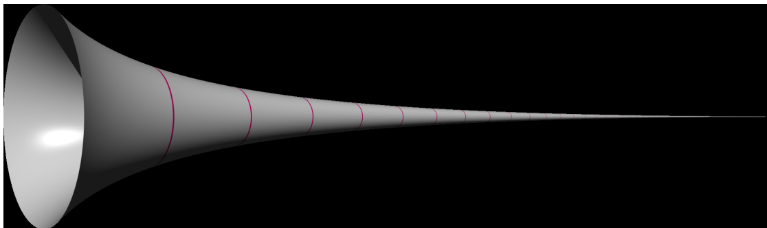
FIGURE 3. Gabriel's Horn.
